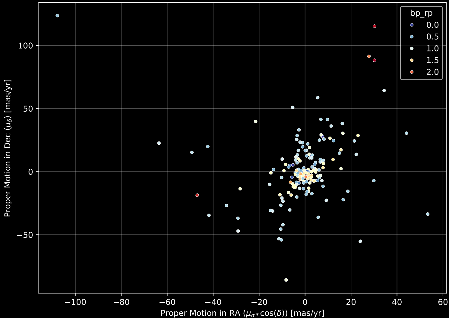
APOGEE DR17 Field: [CVZ_OB15_btx] Proper Motion Diagram (n= 185)
