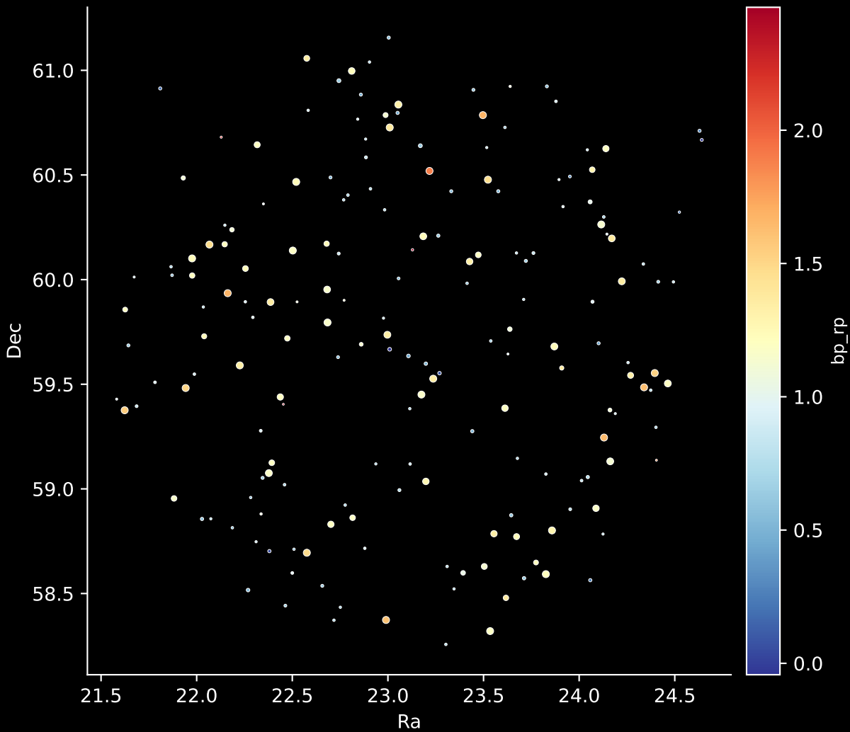
APOGEE DR17 Field: [CVZ_OB15_btx] Stars: 185
