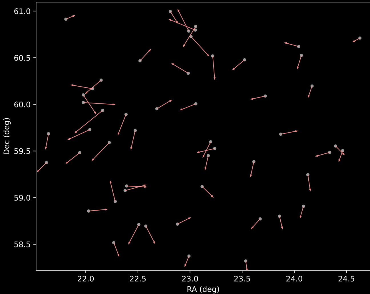
APOGEE DR17 Cluster 7 Proper Motion Vectors (n=52)
