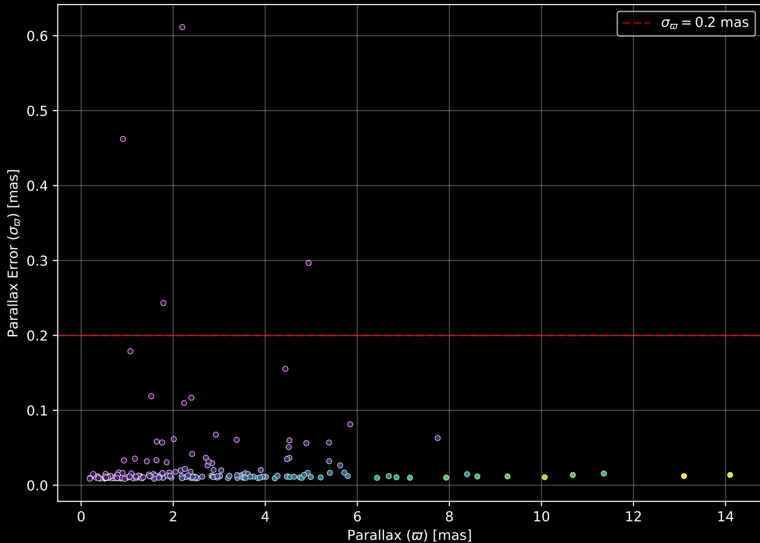
APOGEE DR17 Field: [CVZ_OB15_btx] Parallax Quality (n= 185)
