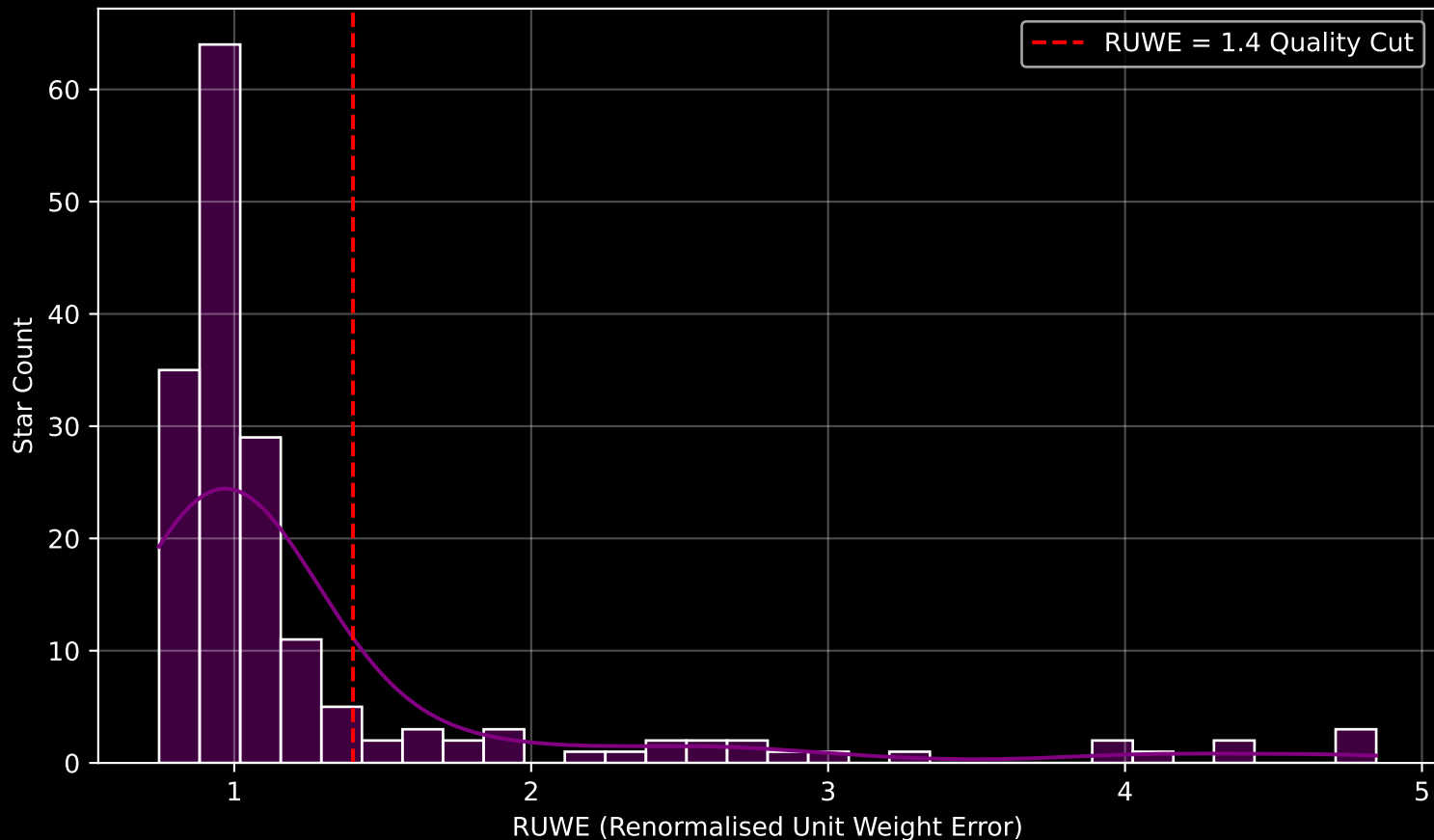
GAPOGEE DR17 Field [CVZ_OB15_btx] RUWE Distribution (n= 173)
