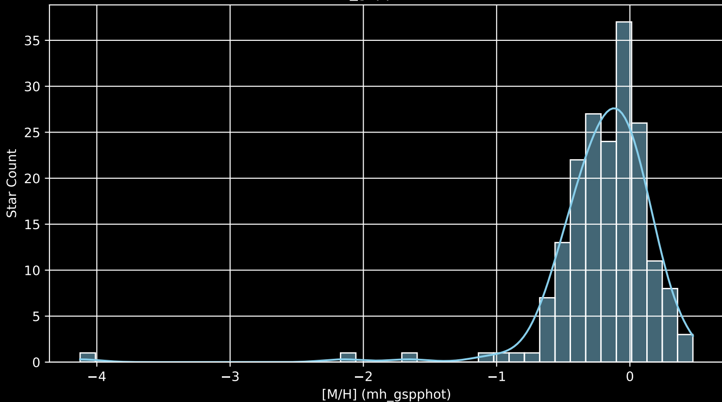
APOGEE DR17 Field: [CVZ_OB15_btx [M/H] (mh_gspphot) (n= 185)
