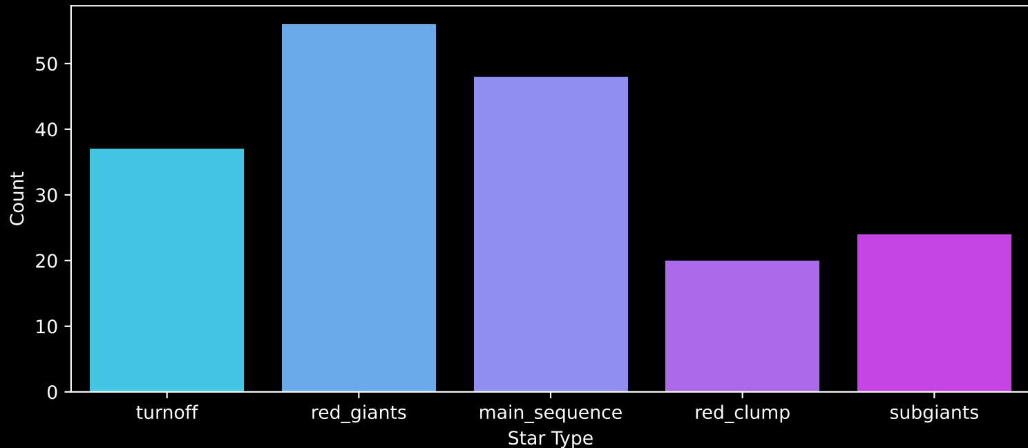
APOGEE DR17 Field: [CVZ_OB15_btx] Count plot of Star Type
